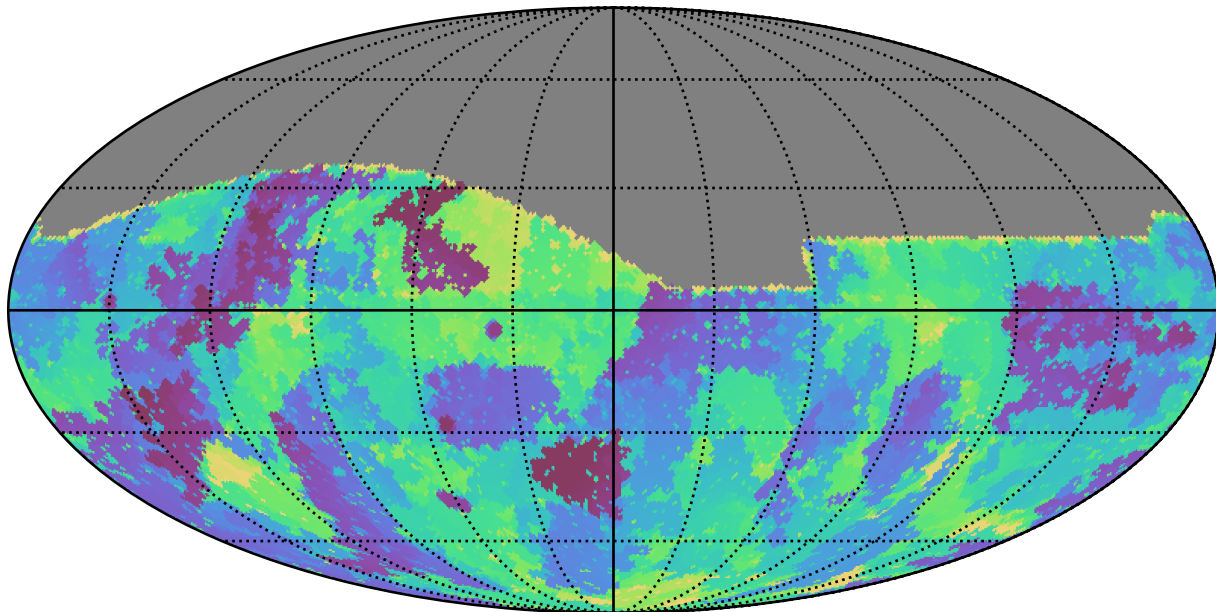
weather_cloudso16v3.4_10yrs All sky g band: Min skyBrightness
