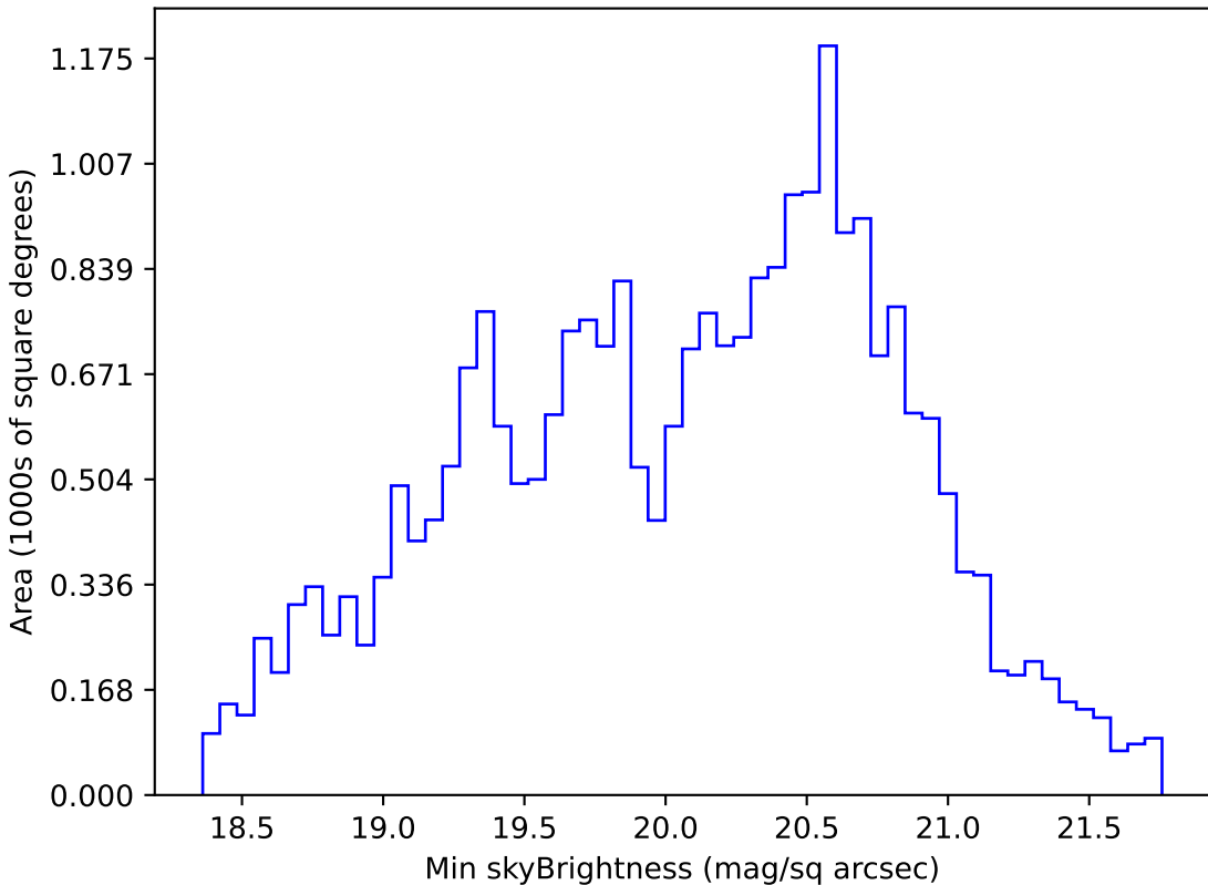
weather_cloudso16v3.4_10yrs All sky g band: Min skyBrightness
