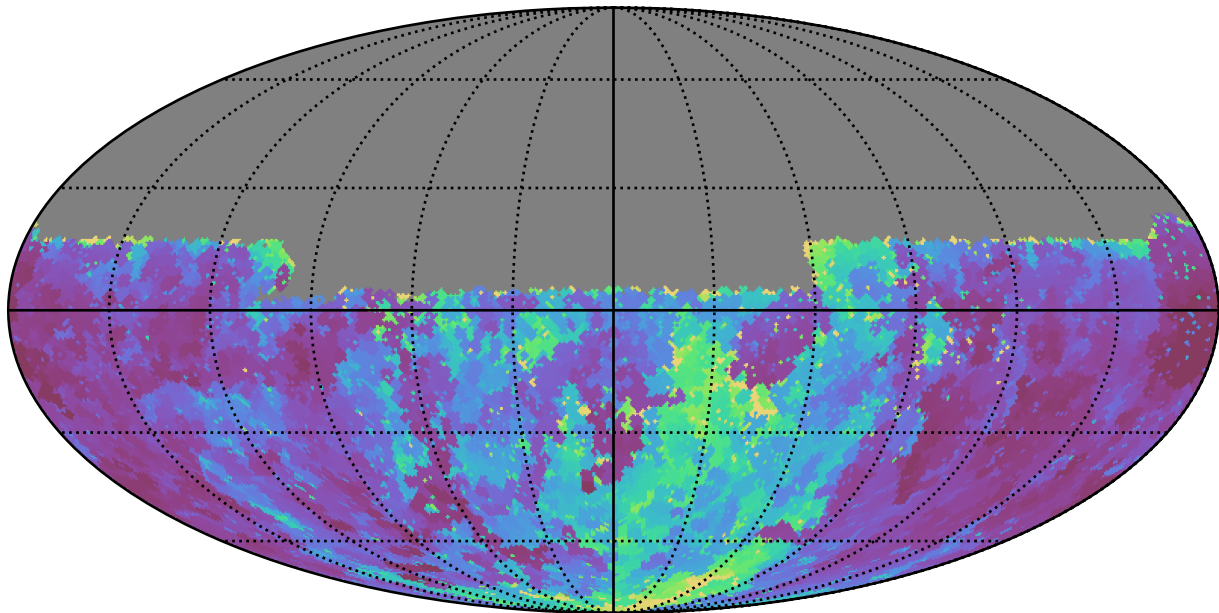
weather_cloudso16v3.4_10yrs Yr 1 u band: Min seeingGeom
