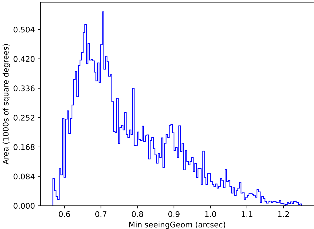
weather_cloudso16v3.4_10yrs Yr 1 u band: Min seeingGeom
