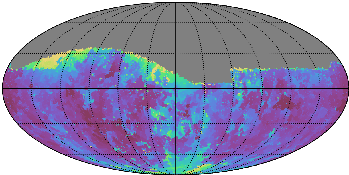
weather_cloudso16v3.4_10yrs Yr 1 g band: Min seeingGeom
