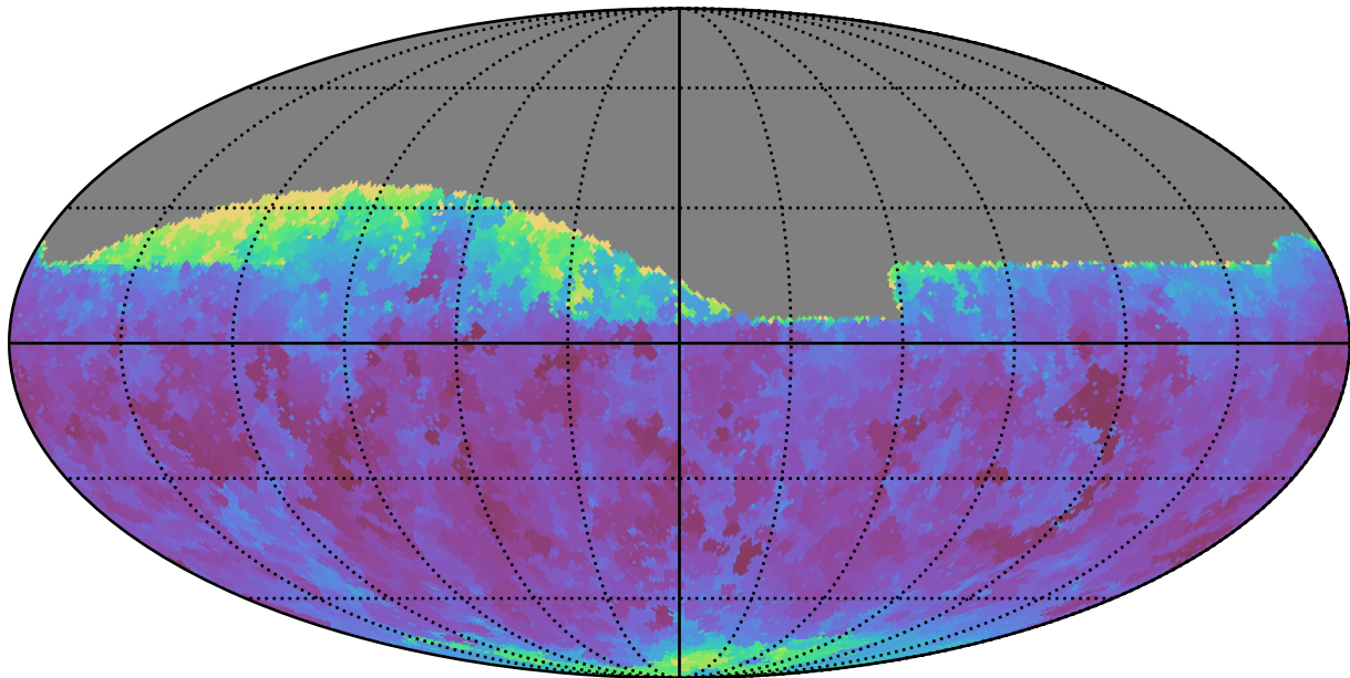
weather_cloudso16v3.4_10yrs Yr 1 all bands: Min seeingGeom
