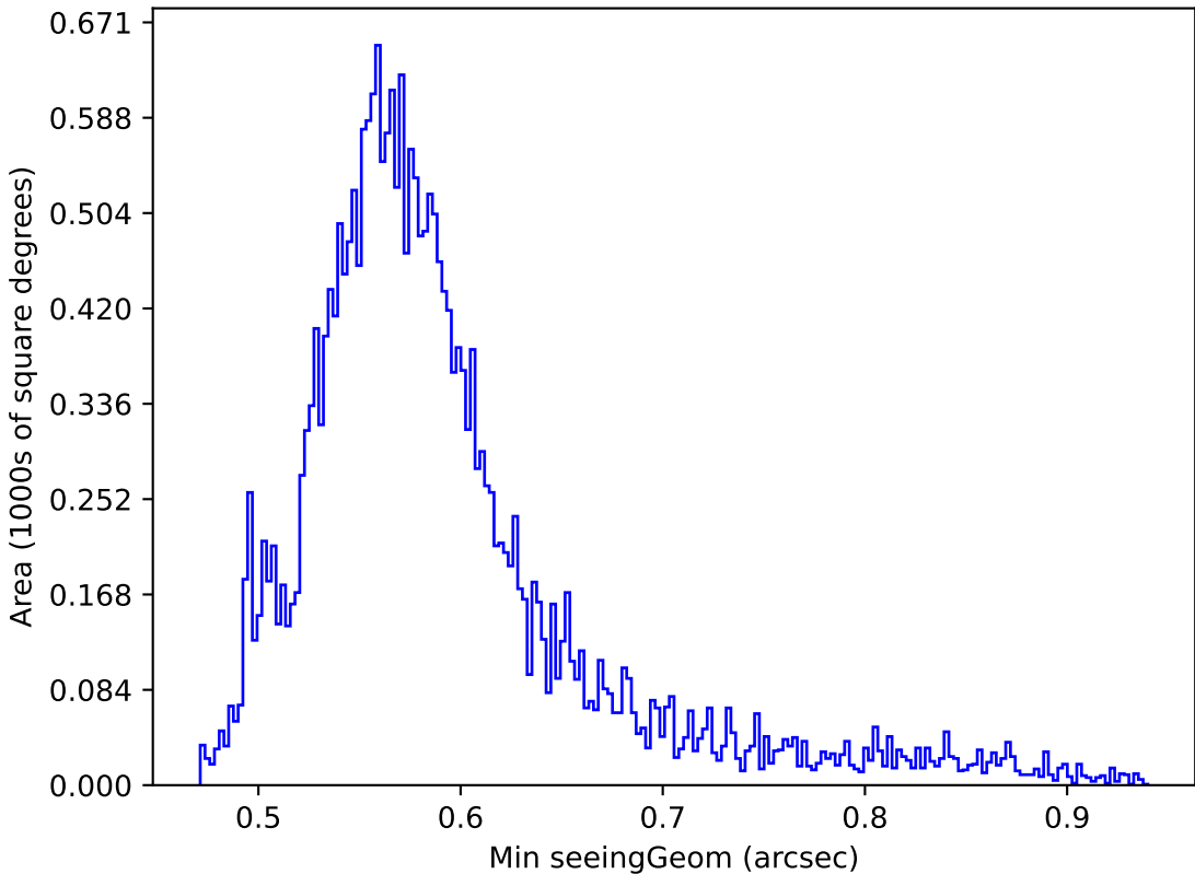
weather_cloudso16v3.4_10yrs Yr 1 all bands: Min seeingGeom
