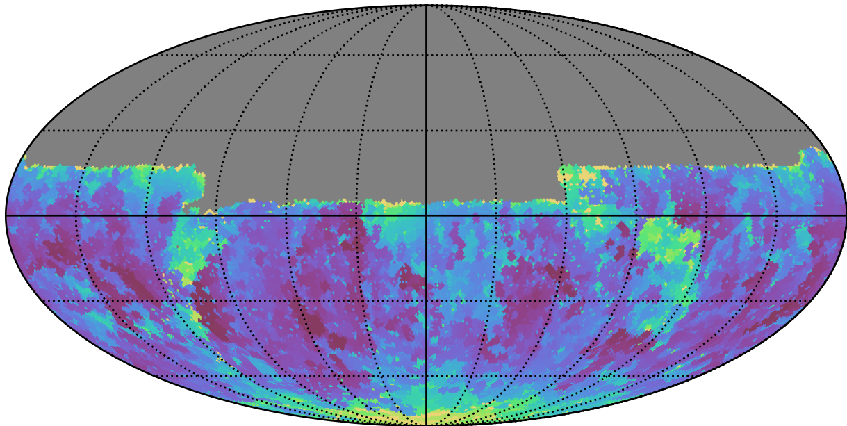
weather_cloudso16v3.4_10yrs Yr 1 y band: Min seeingEff
