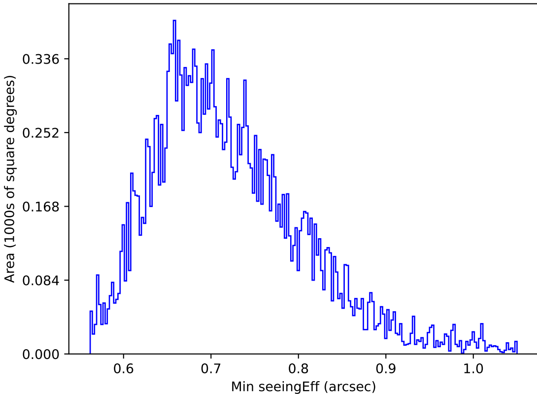
weather_cloudso16v3.4_10yrs Yr 1 y band: Min seeingEff
