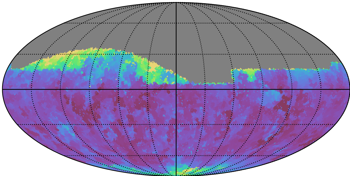
weather_cloudso16v3.4_10yrs Yr 1 r band: Min seeingEff
