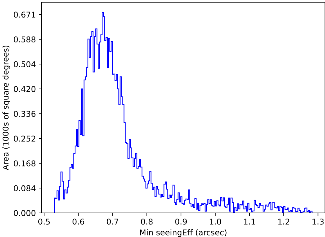
weather_cloudso16v3.4_10yrs Yr 1 r band: Min seeingEff
