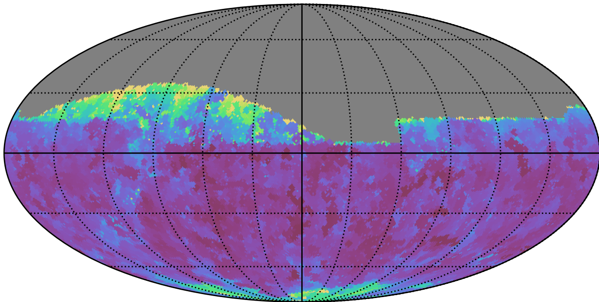
weather_cloudso16v3.4_10yrs Yr 1 i band: Min seeingEff
