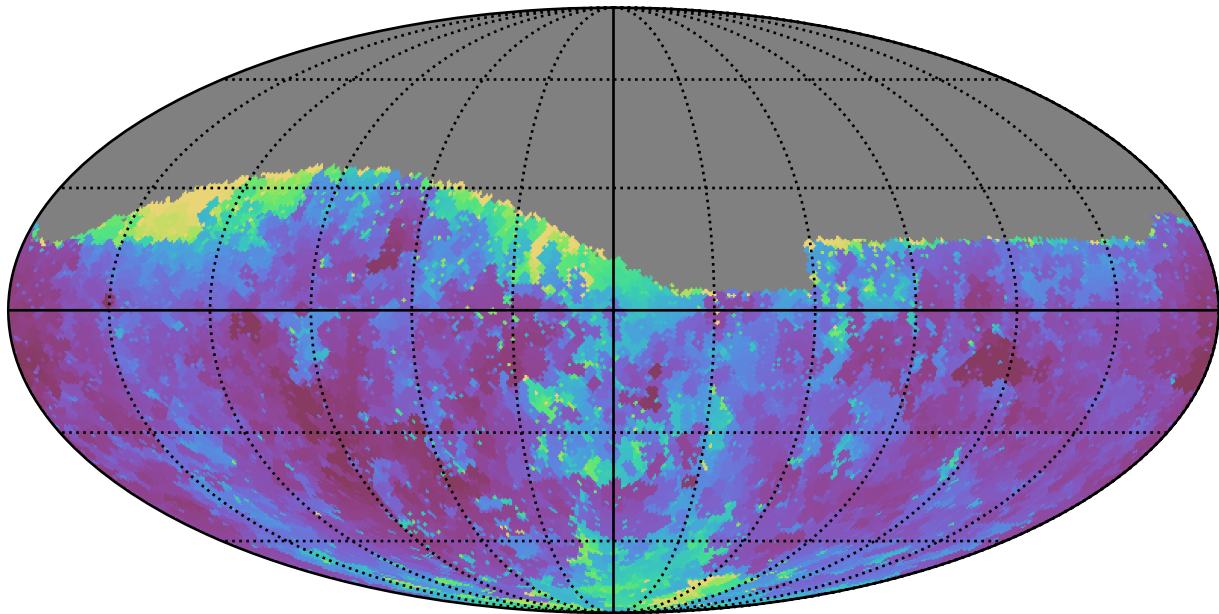
weather_cloudso16v3.4_10yrs Yr 1 g band: Min seeingEff
