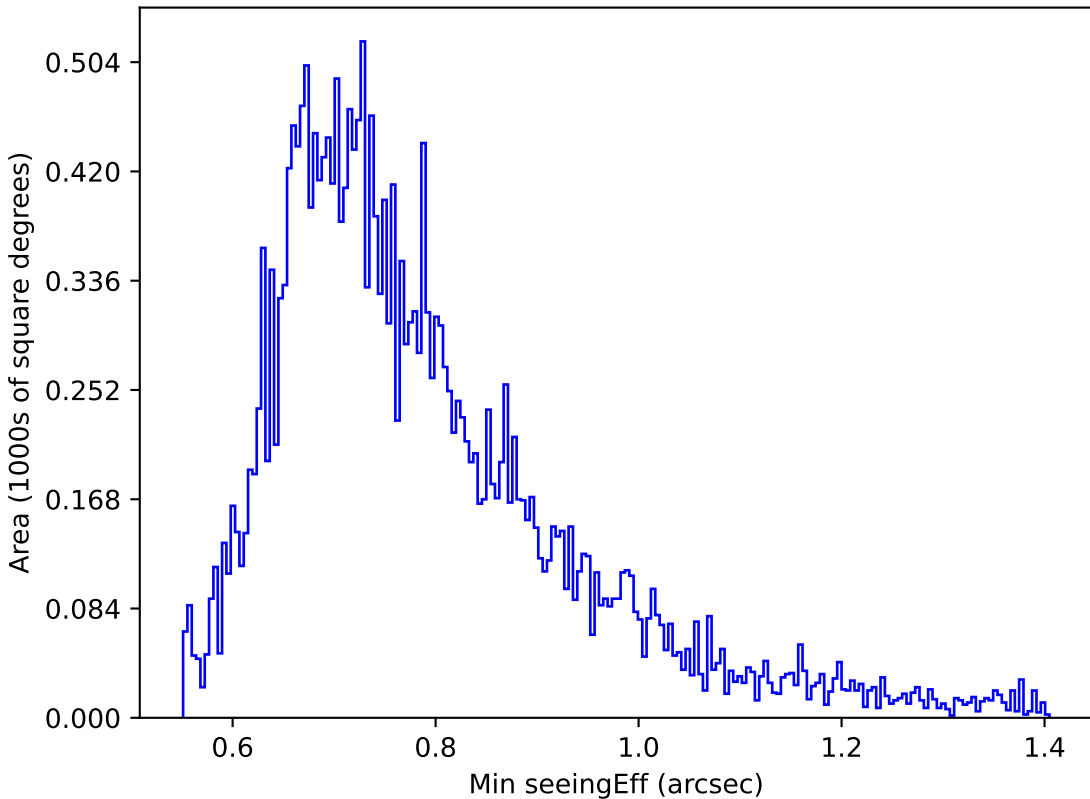
weather_cloudso16v3.4_10yrs Yr 1 g band: Min seeingEff
