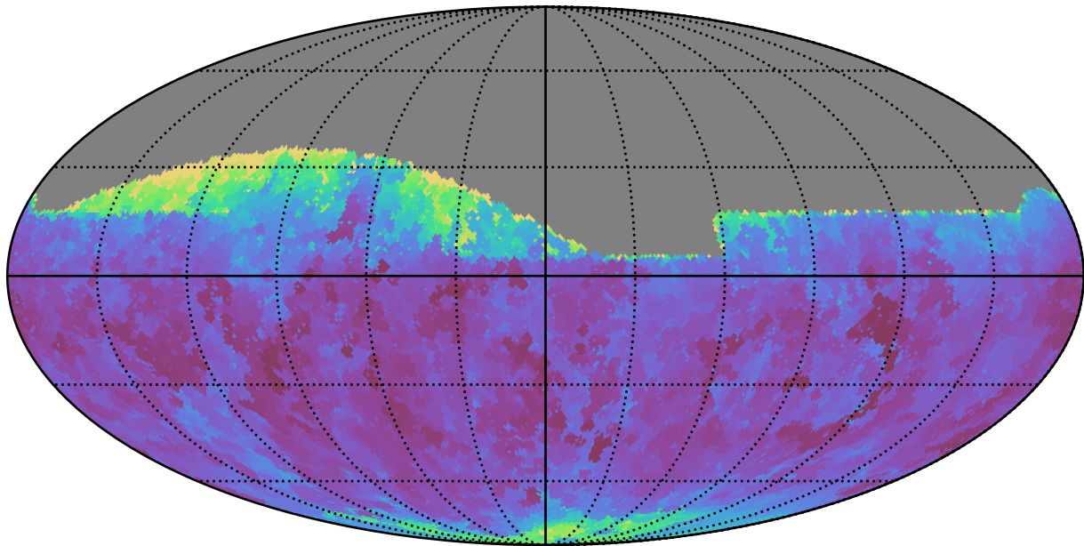
weather_cloudso16v3.4_10yrs Yr 1 all bands: Min seeingEff
