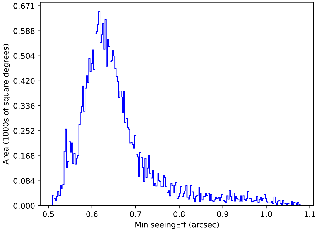
weather_cloudso16v3.4_10yrs Yr 1 all bands: Min seeingEff
