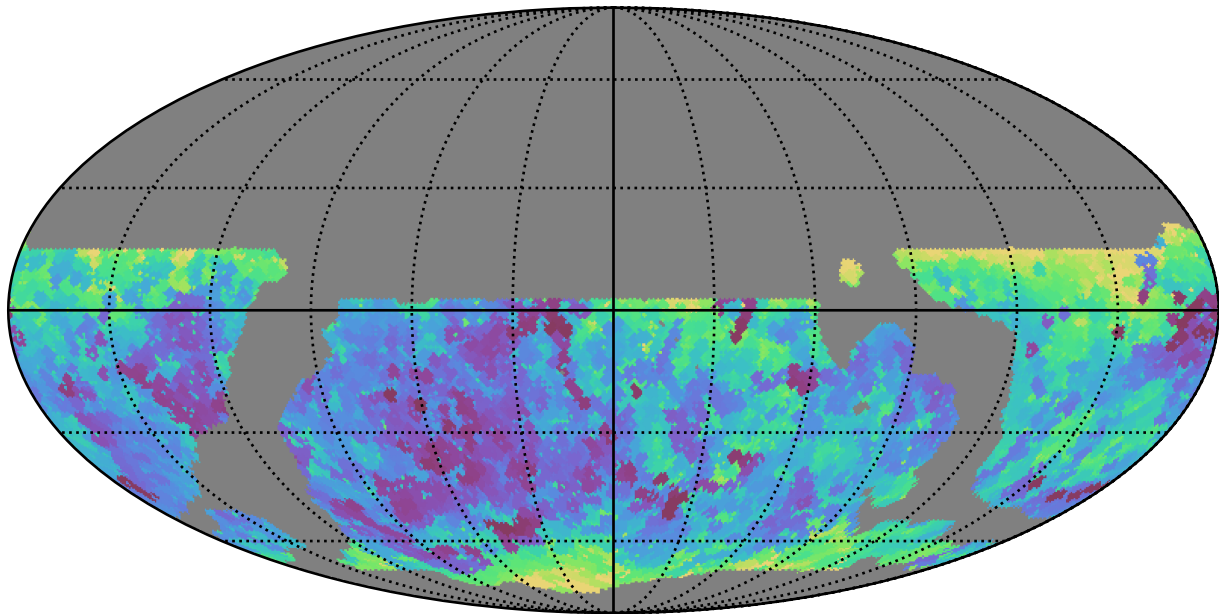
weather_cloudso16v3.4_10yrs WFD z band: Min seeingEff
