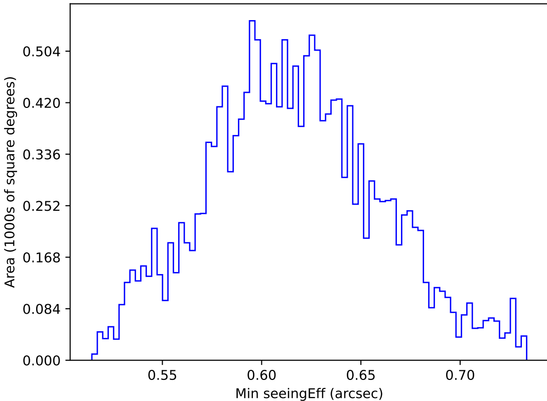
weather_cloudso16v3.4_10yrs WFD z band: Min seeingEff
