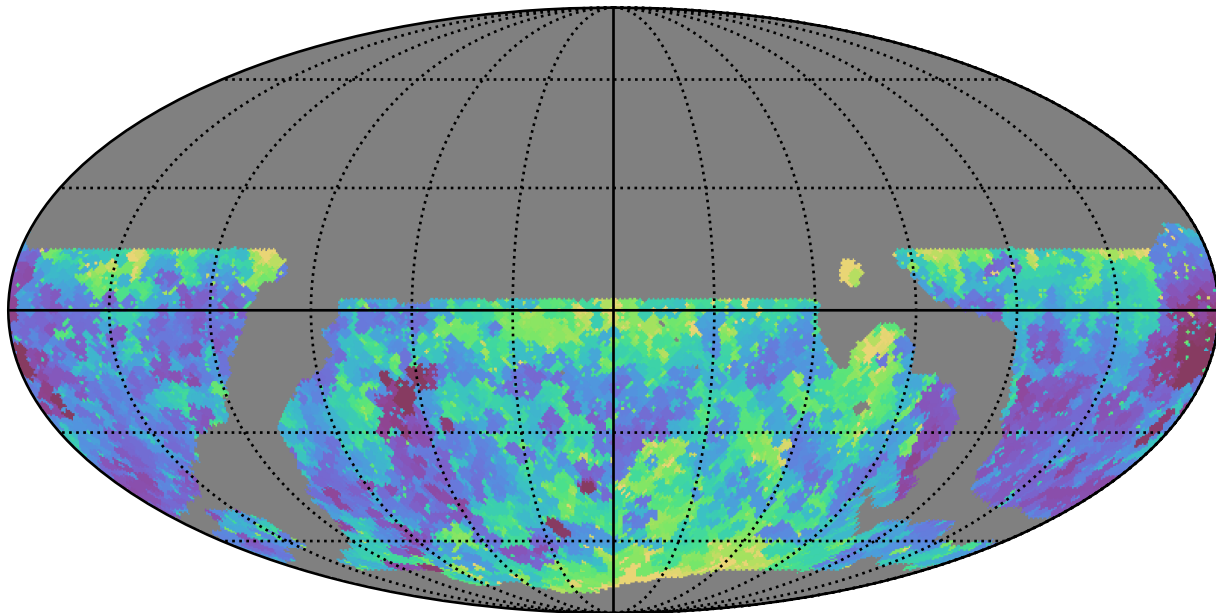
weather_cloudso16v3.4_10yrs WFD u band: Min seeingEff
