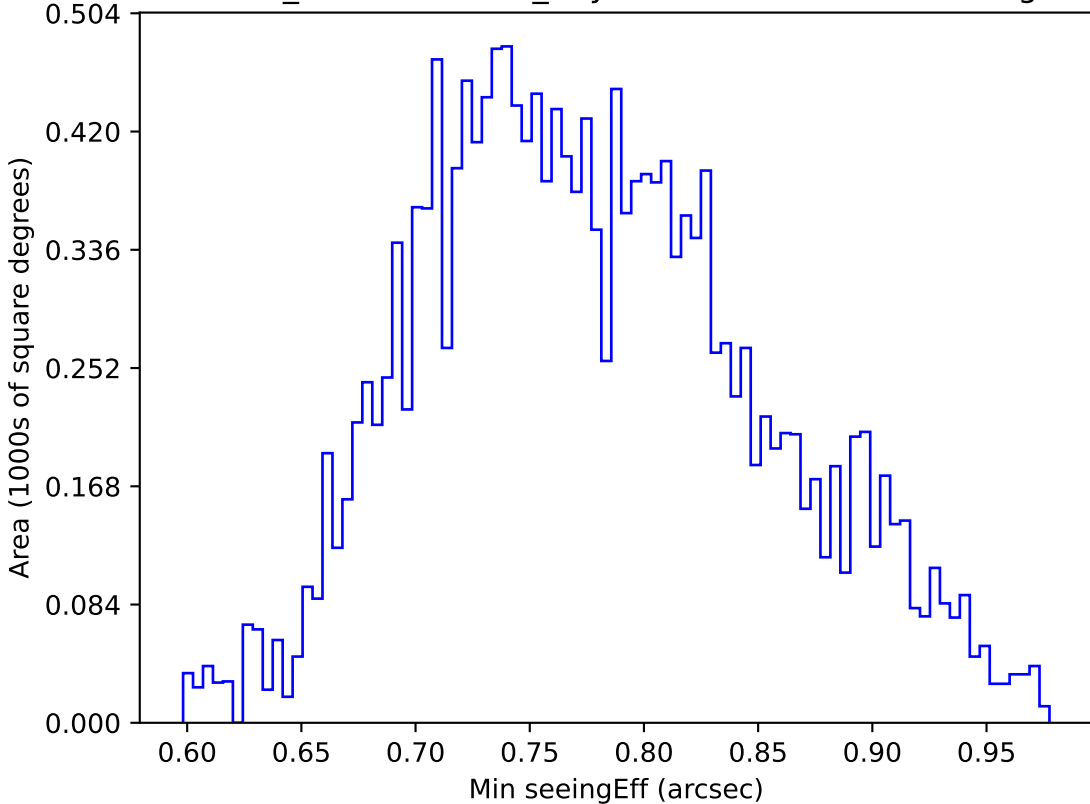
weather_cloudso16v3.4_10yrs WFD u band: Min seeingEff
