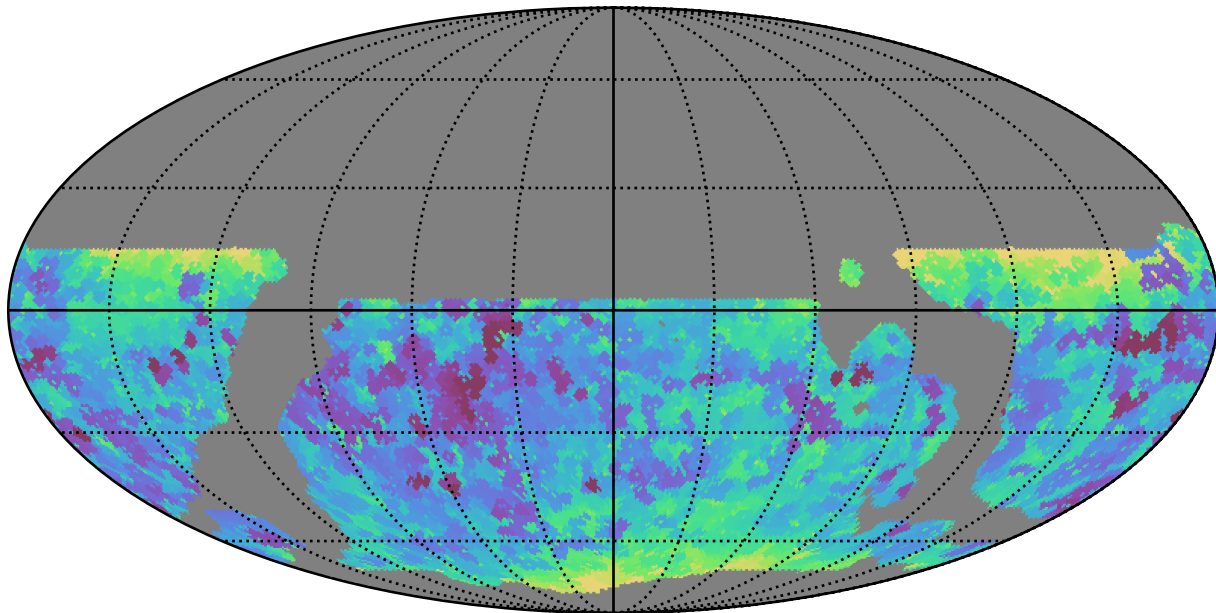
weather_cloudso16v3.4_10yrs WFD r band: Min seeingEff
