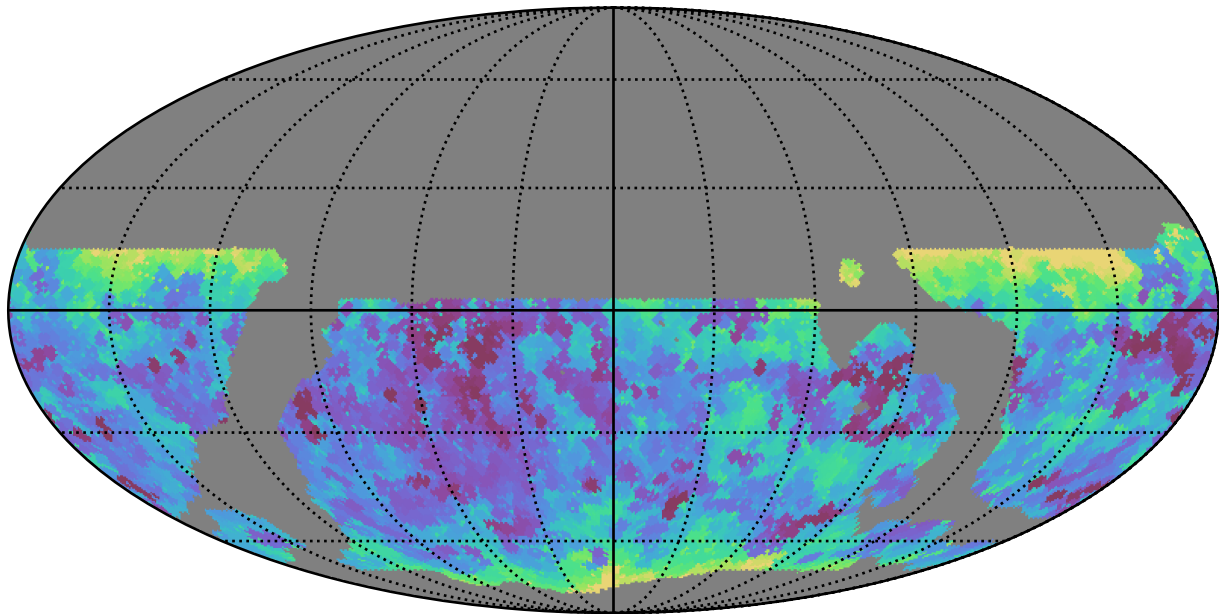
weather_cloudso16v3.4_10yrs WFD all bands: Min seeingEff
