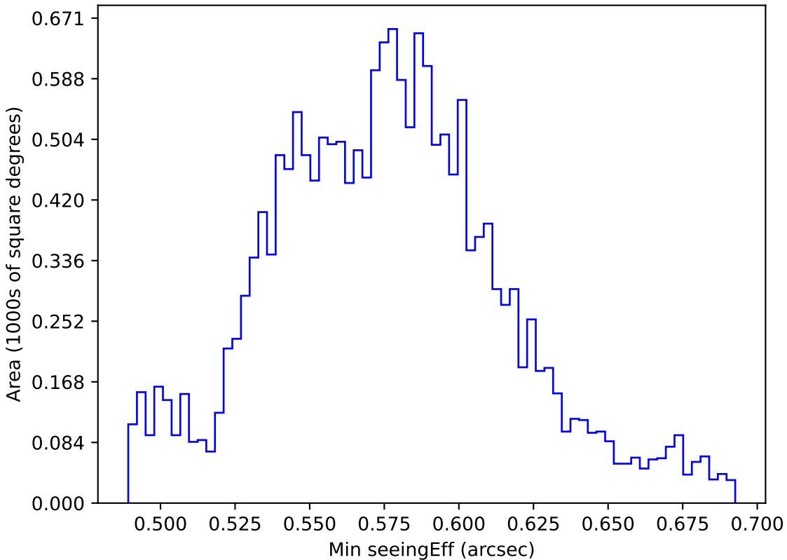
weather_cloudso16v3.4_10yrs WFD all bands: Min seeingEff
