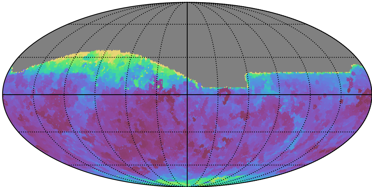
weather_cloudso16v3.4_10yrs All sky z band: Min seeingEff
