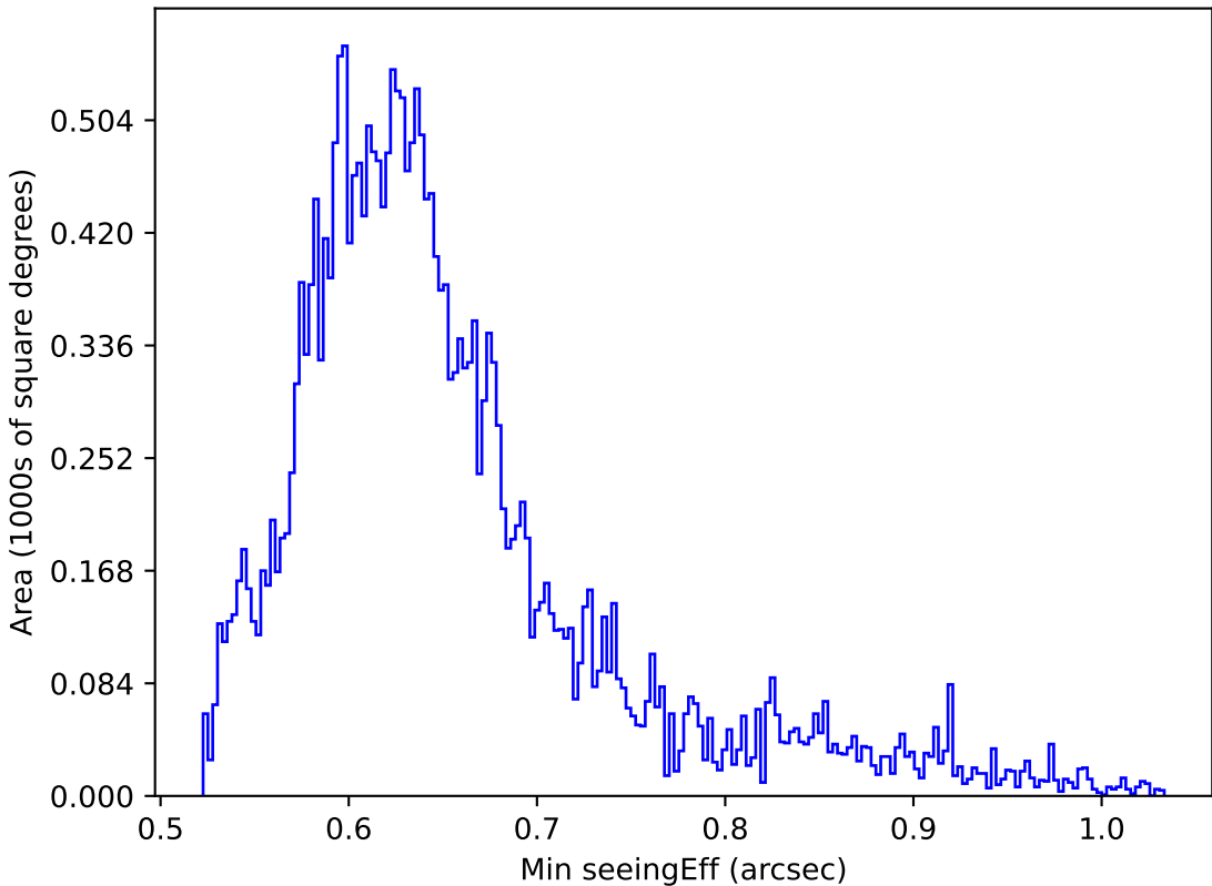
weather_cloudso16v3.4_10yrs All sky z band: Min seeingEff
