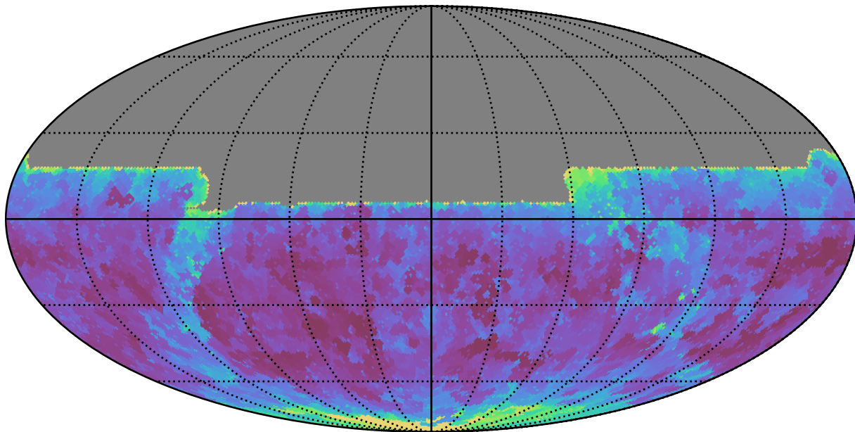
weather_cloudso16v3.4_10yrs All sky y band: Min seeingEff
