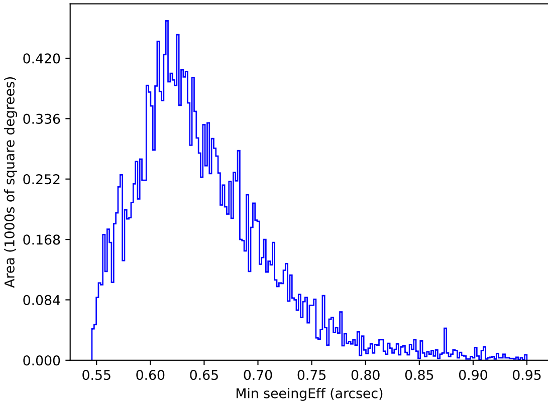
weather_cloudso16v3.4_10yrs All sky y band: Min seeingEff
