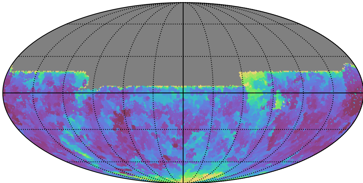
weather_cloudso16v3.4_10yrs All sky u band: Min seeingEff
