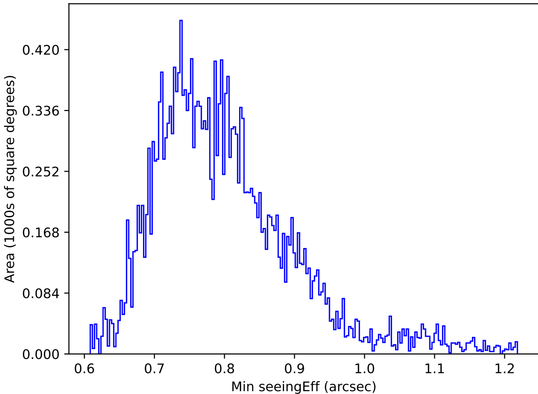
weather_cloudso16v3.4_10yrs All sky u band: Min seeingEff
