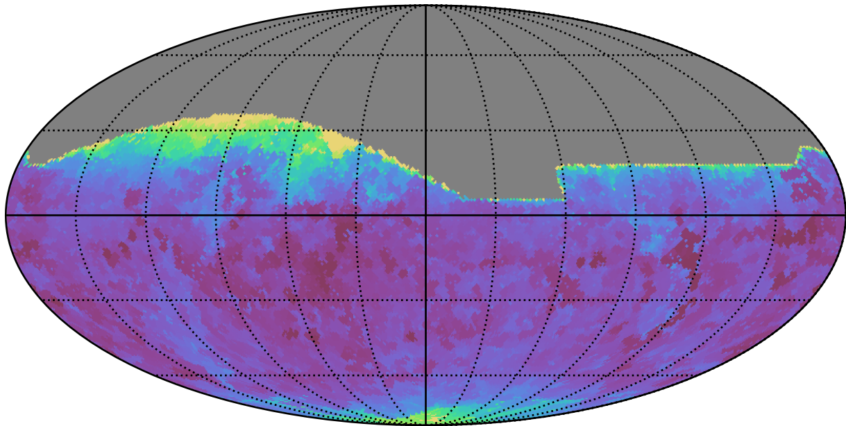
weather_cloudso16v3.4_10yrs All sky r band: Min seeingEff
