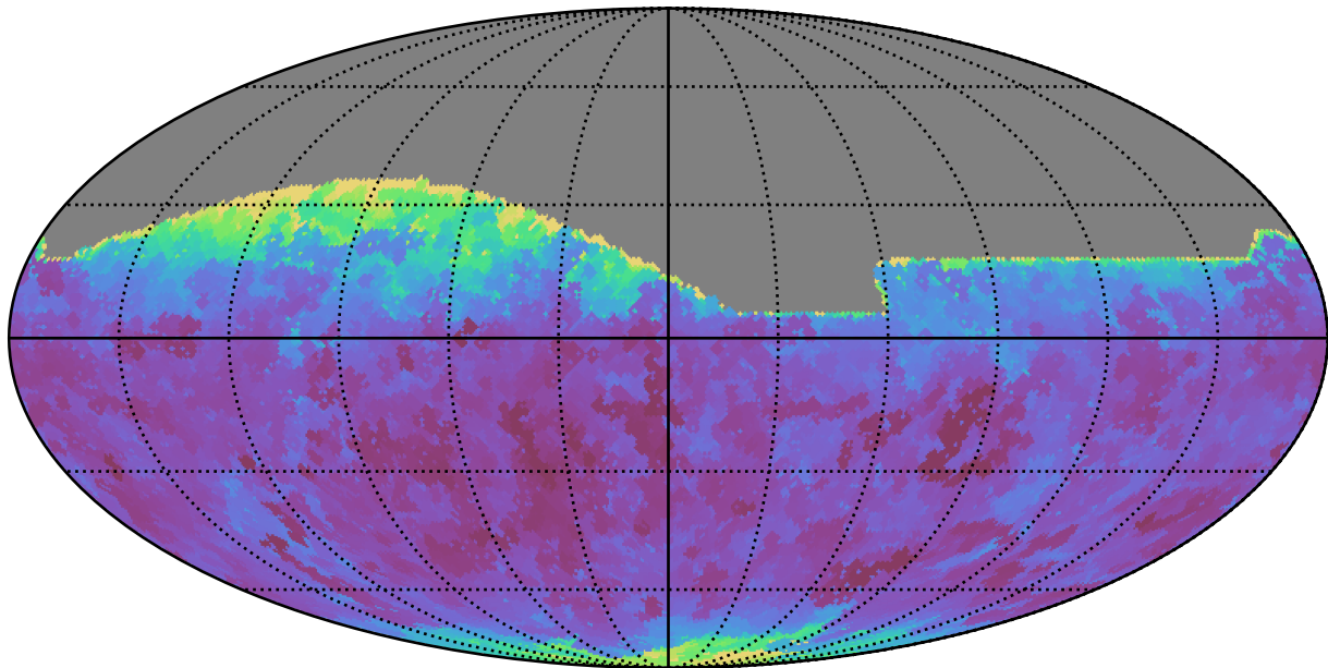
weather_cloudso16v3.4_10yrs All sky i band: Min seeingEff
