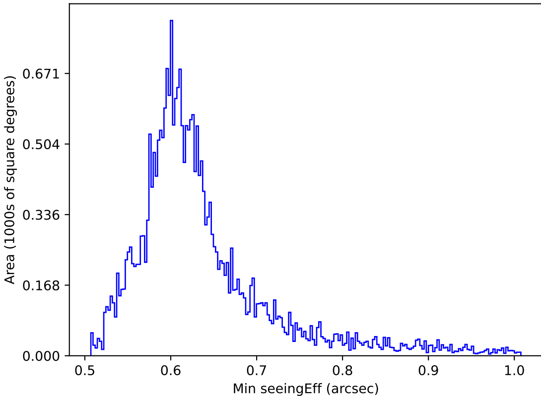
weather_cloudso16v3.4_10yrs All sky i band: Min seeingEff
