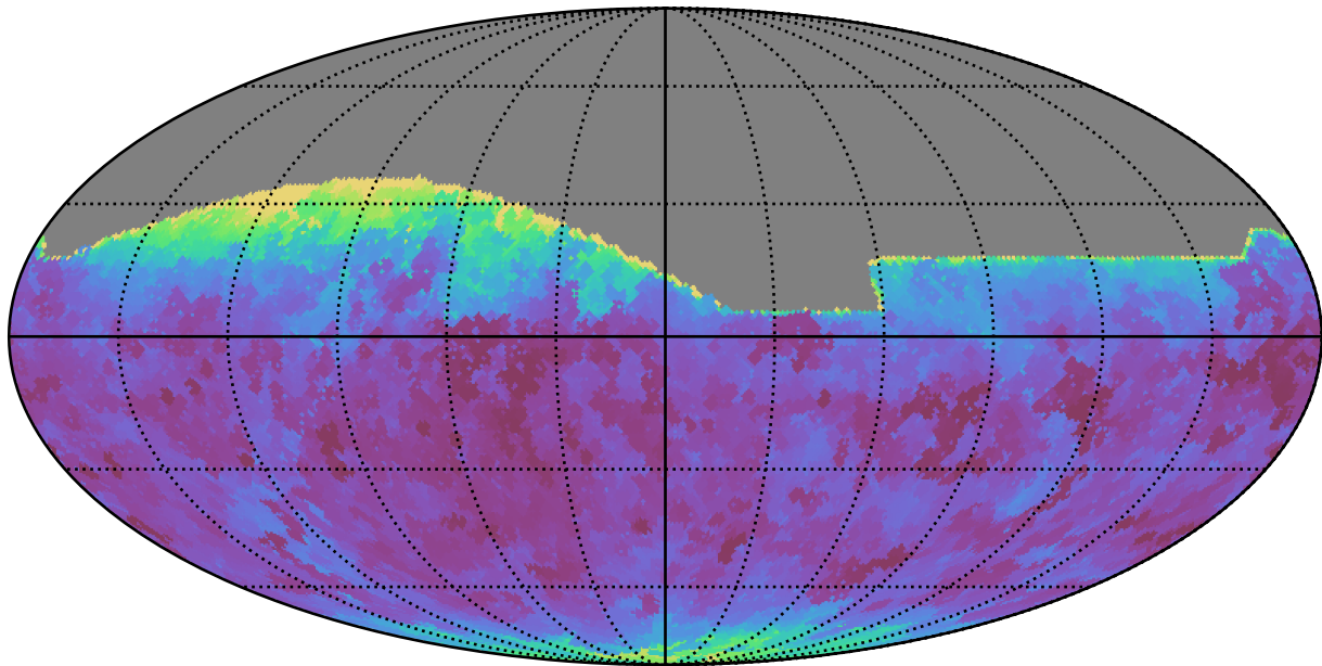
weather_cloudso16v3.4_10yrs All sky all bands: Min seeingEff
