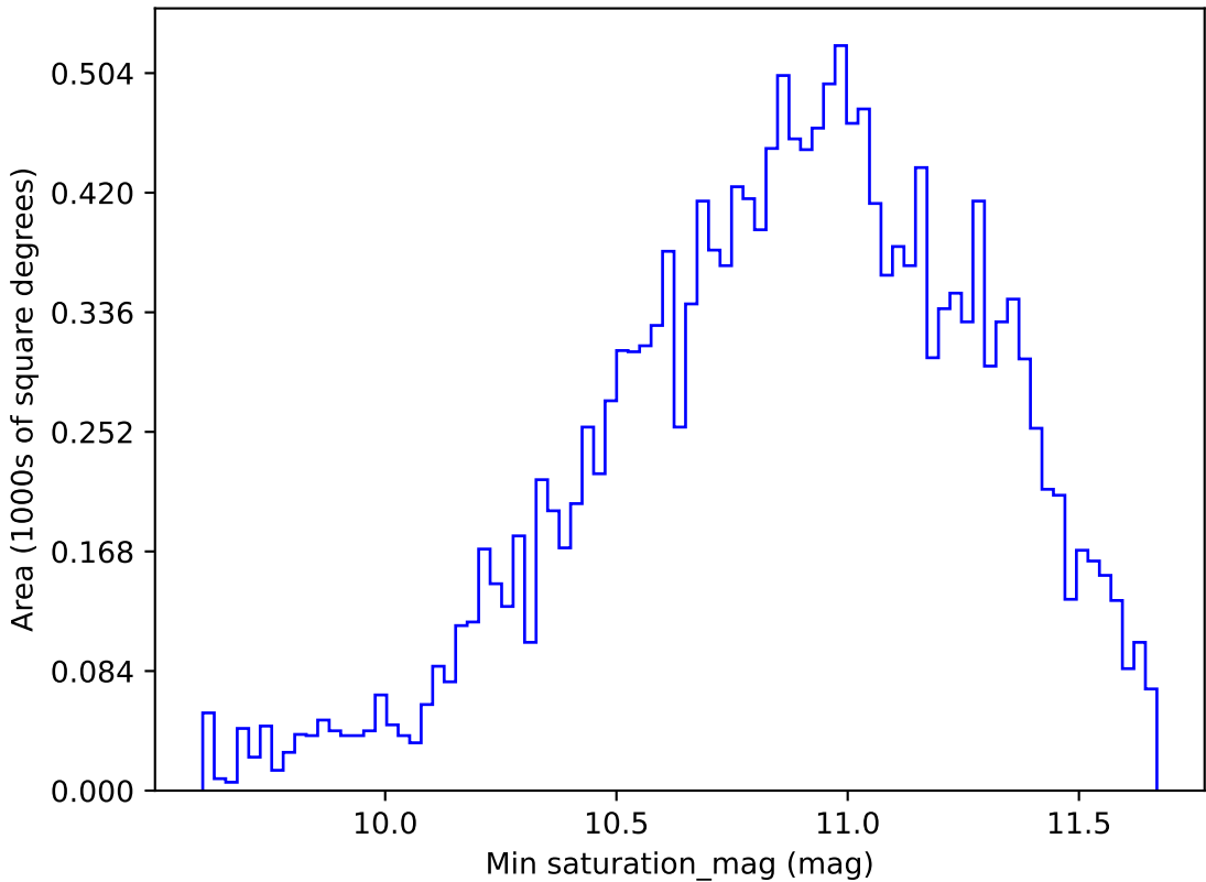
weather_cloudso16v3.4_10yrs WFD all bands: Min saturation_mag
