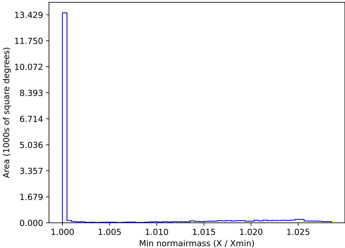
weather_cloudso16v3.4_10yrs WFD all bands: Min normairmass
