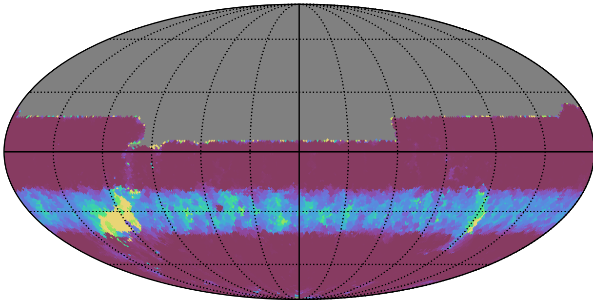
weather_cloudso16v3.4_10yrs All sky u band: Min normairmass
