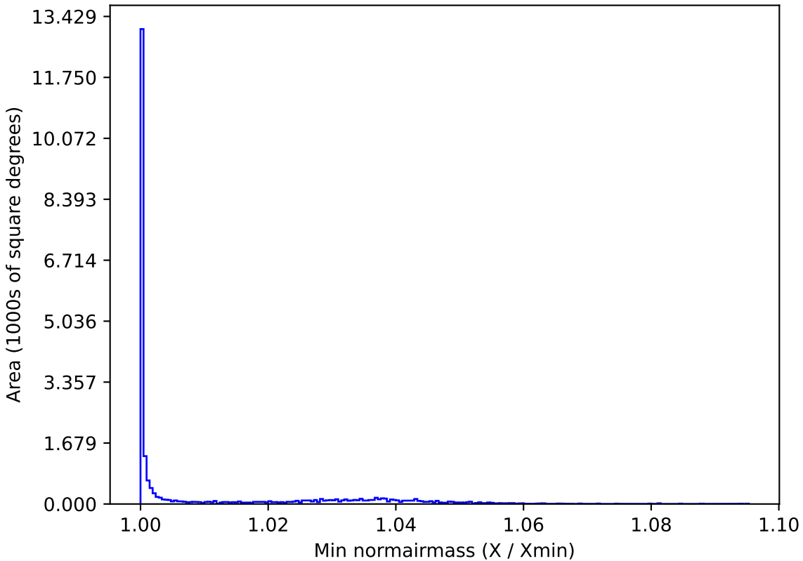
weather_cloudso16v3.4_10yrs All sky u band: Min normairmass
