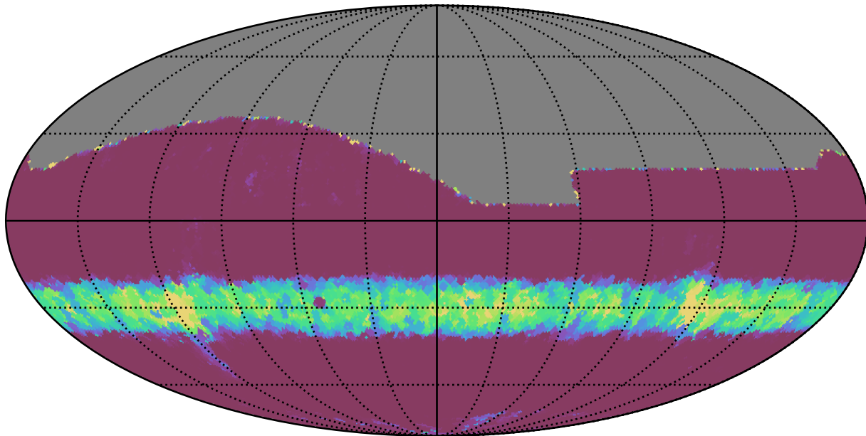
weather_cloudso16v3.4_10yrs All sky r band: Min normairmass
