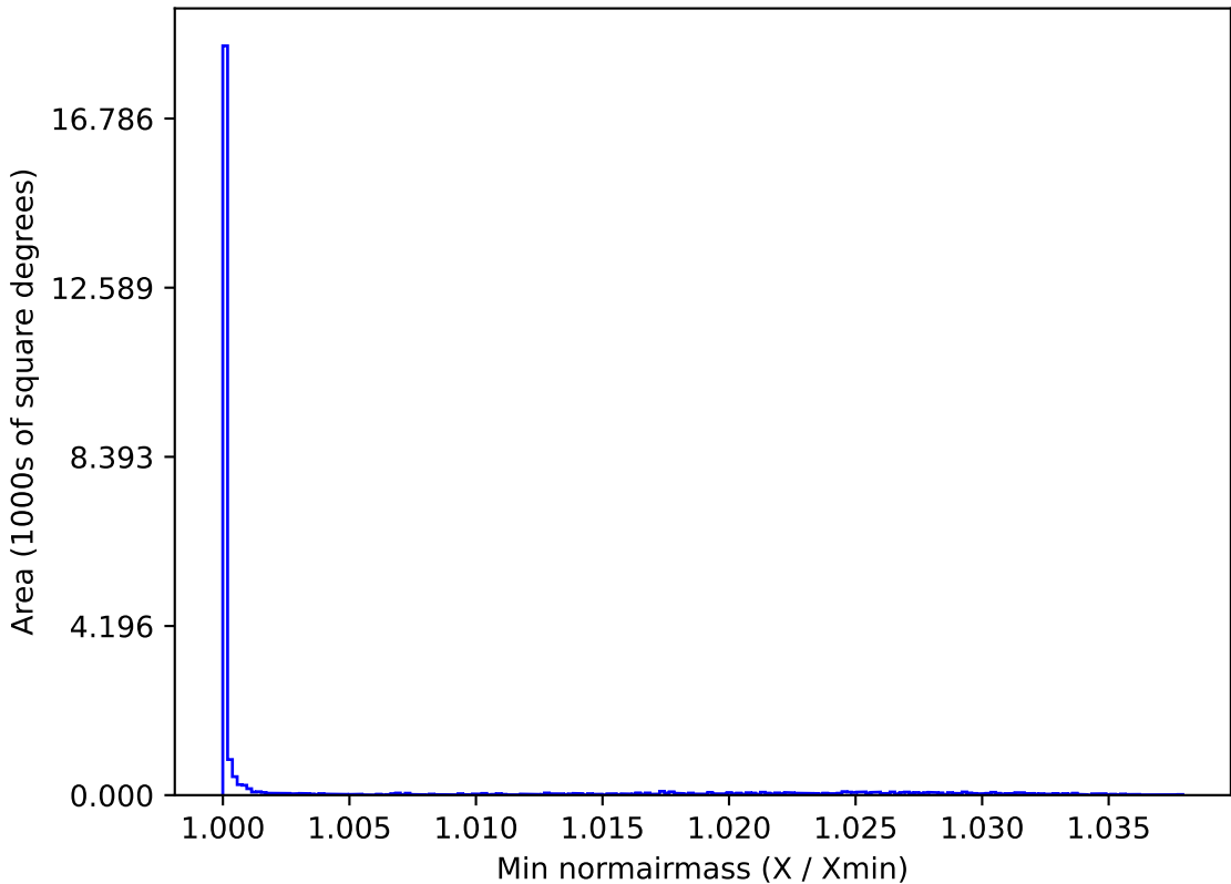
weather_cloudso16v3.4_10yrs All sky r band: Min normairmass
