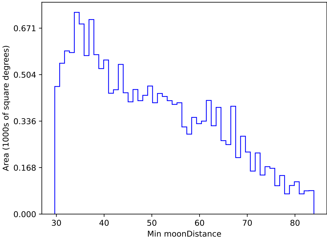
weather_cloudso16v3.4_10yrs WFD u band: Min moonDistance
