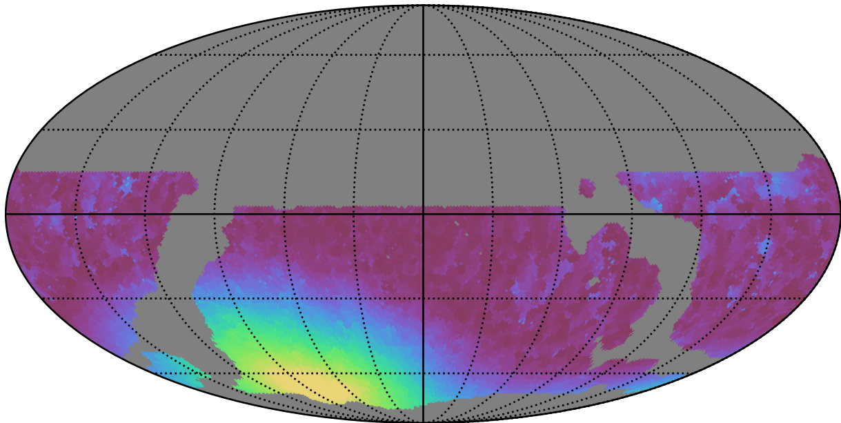
weather_cloudso16v3.4_10yrs WFD r band: Min moonDistance
