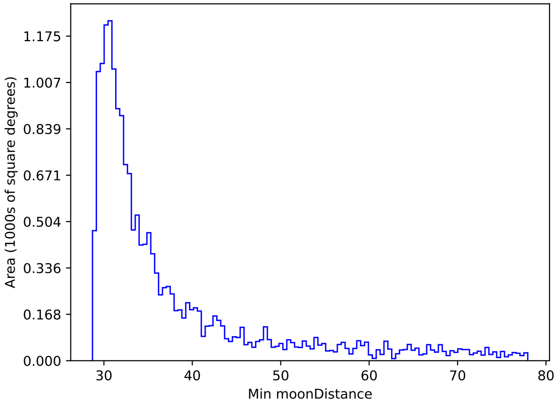
weather_cloudso16v3.4_10yrs WFD r band: Min moonDistance
