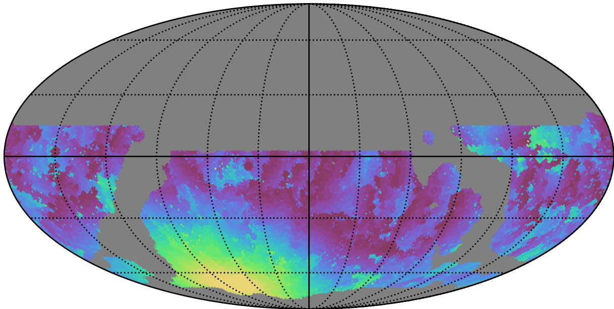
weather_cloudso16v3.4_10yrs WFD g band: Min moonDistance
