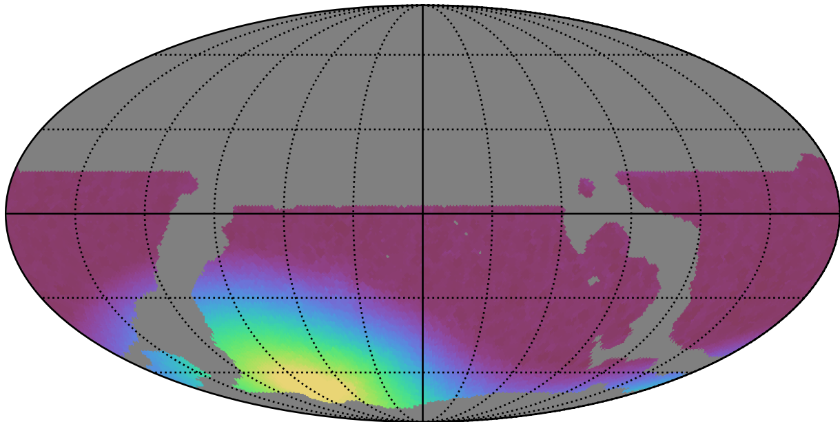
weather_cloudso16v3.4_10yrs WFD all bands: Min moonDistance
