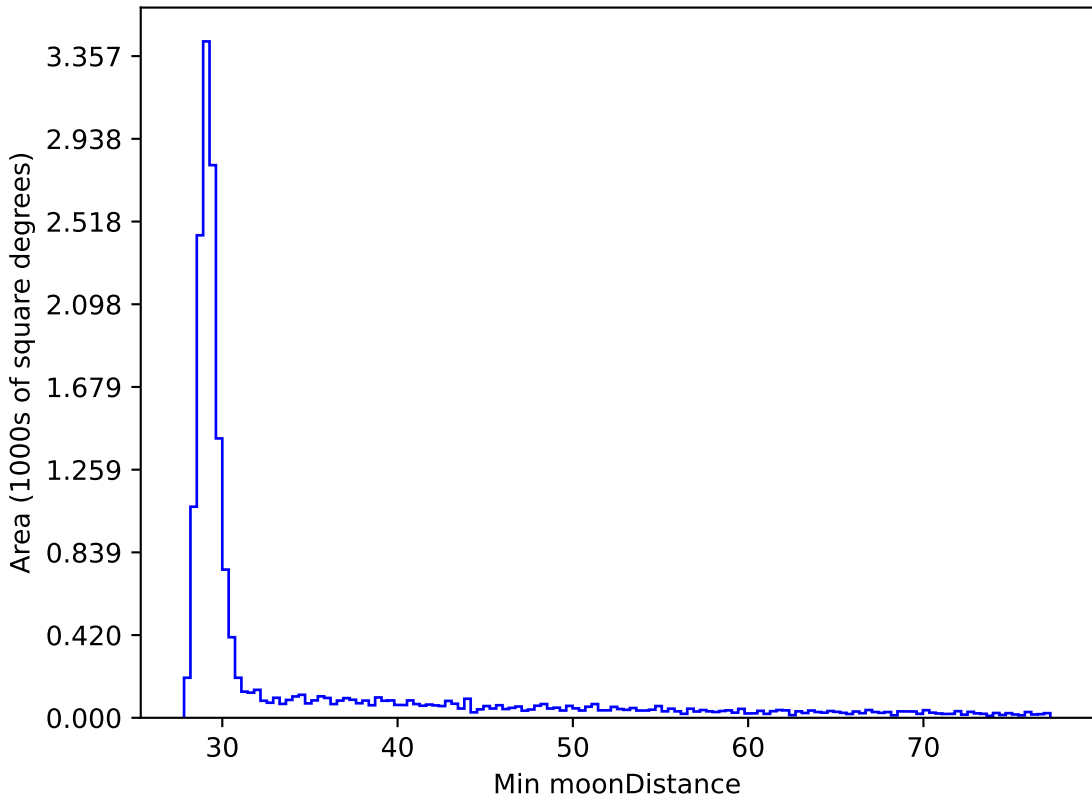
weather_cloudso16v3.4_10yrs WFD all bands: Min moonDistance
