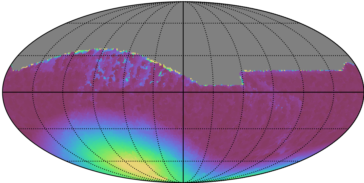
weather_cloudso16v3.4_10yrs All sky z band: Min moonDistance
