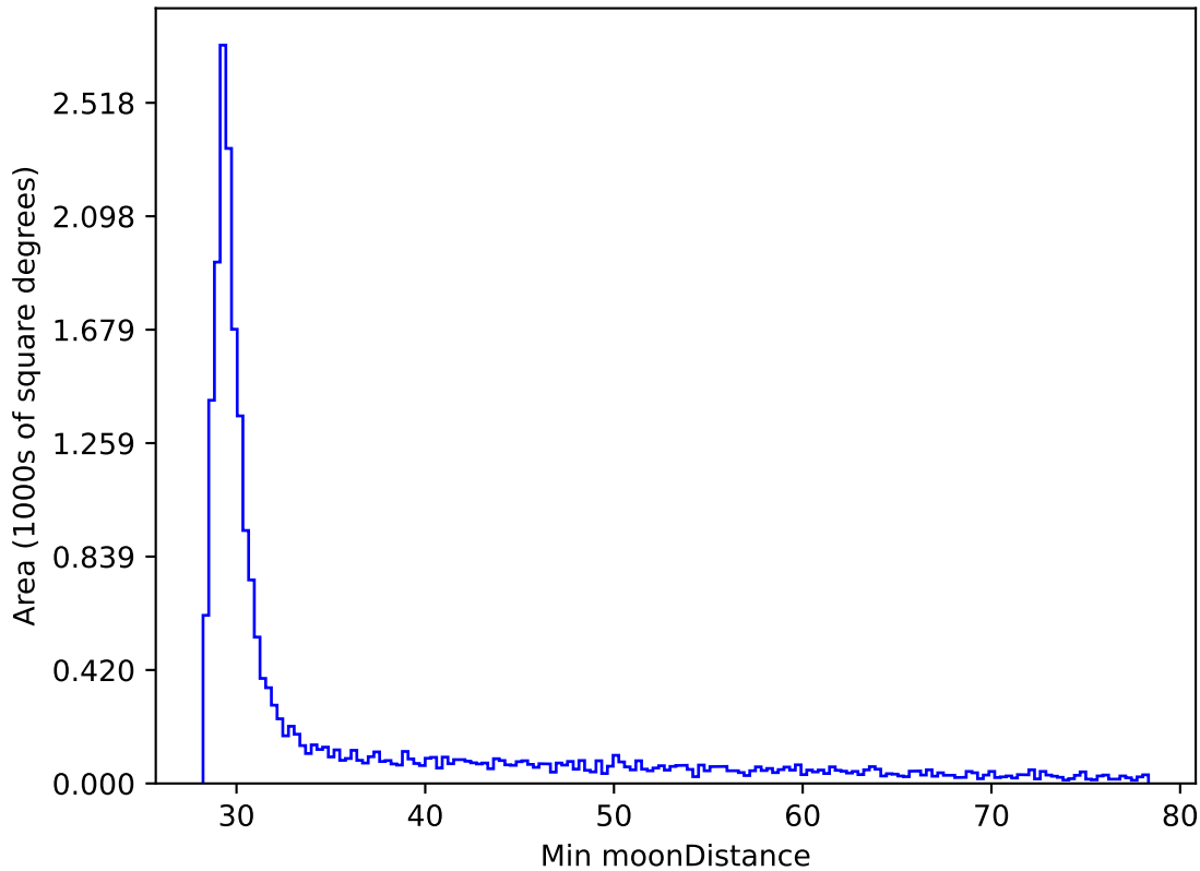
weather_cloudso16v3.4_10yrs All sky y band: Min moonDistance
