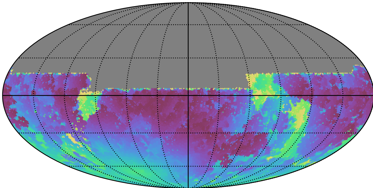
weather_cloudso16v3.4_10yrs All sky u band: Min moonDistance
