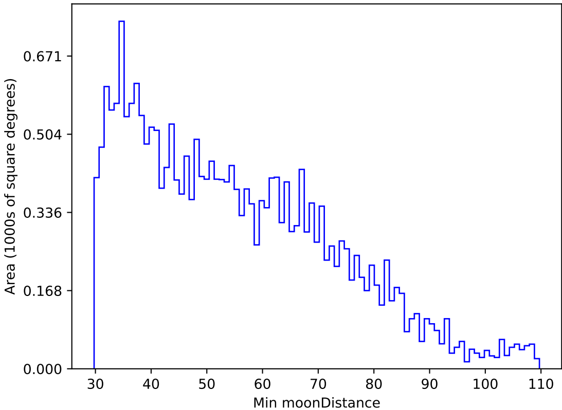
weather_cloudso16v3.4_10yrs All sky u band: Min moonDistance
