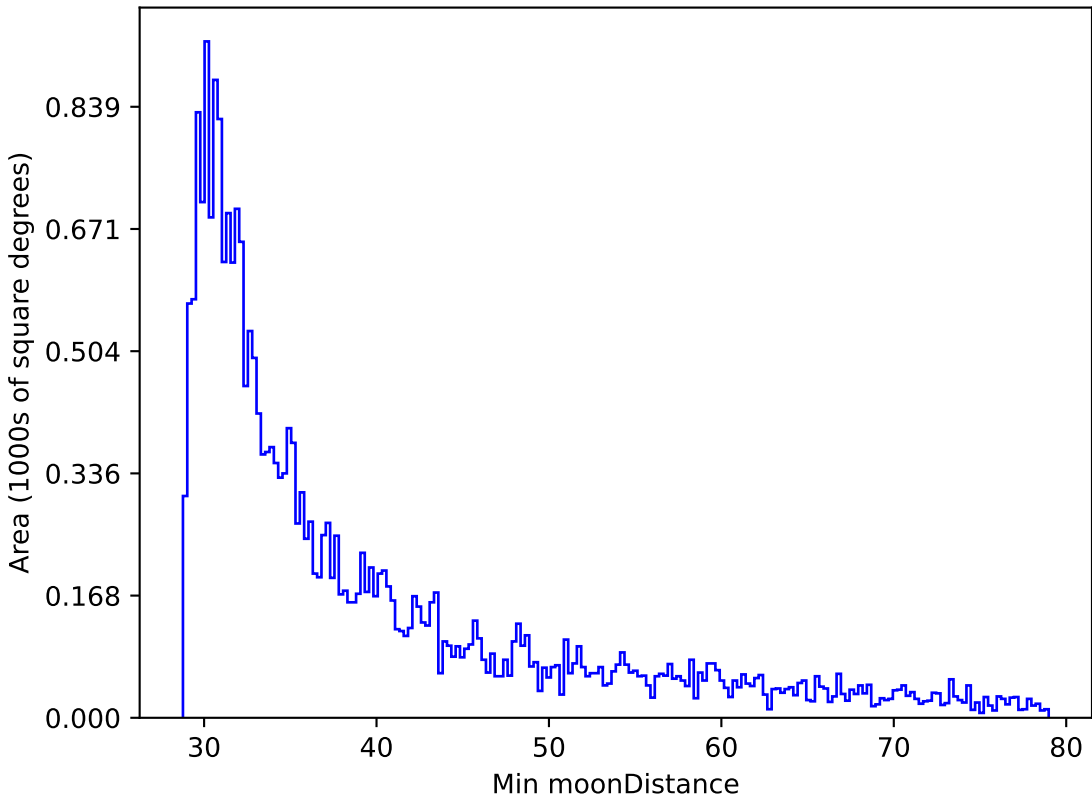
weather_cloudso16v3.4_10yrs All sky r band: Min moonDistance
